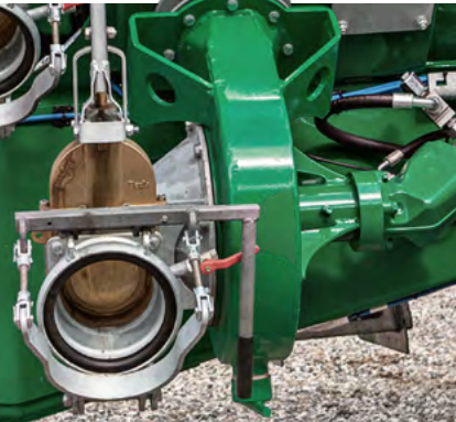
Side-mounted filling pump* Side-mounted filling pump with manual slide valve and quick hose coupling.
